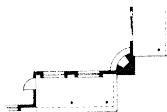
PORCH (ROOF OPTION 1)
